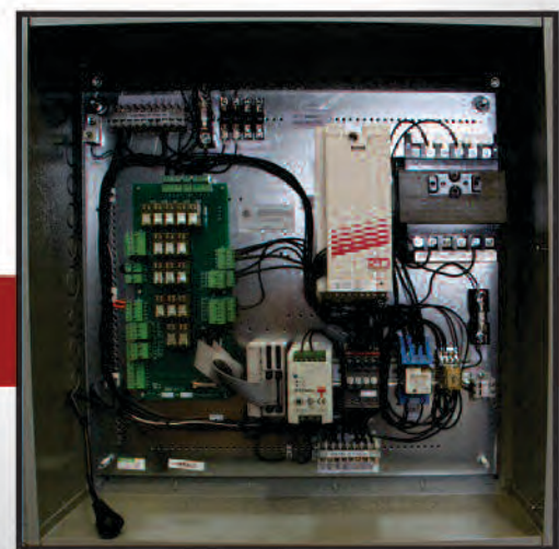
Controller Cabinet
